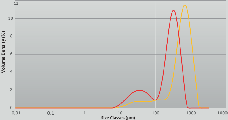
Comparative particle size distribution for All Purpose Black
