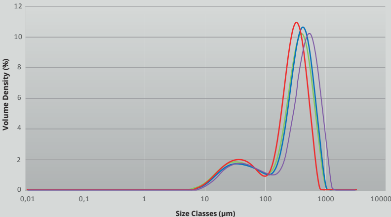
Comparative particle size distribution in espresso grind setting
