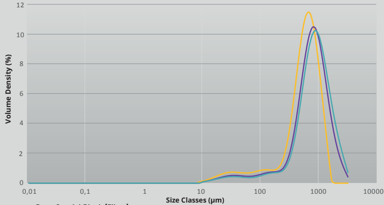
Comparative particle size distribution in filter grind setting
